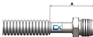
Metal Face Seal Male*
